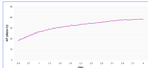
Antenna factor HyperLOG 4040
